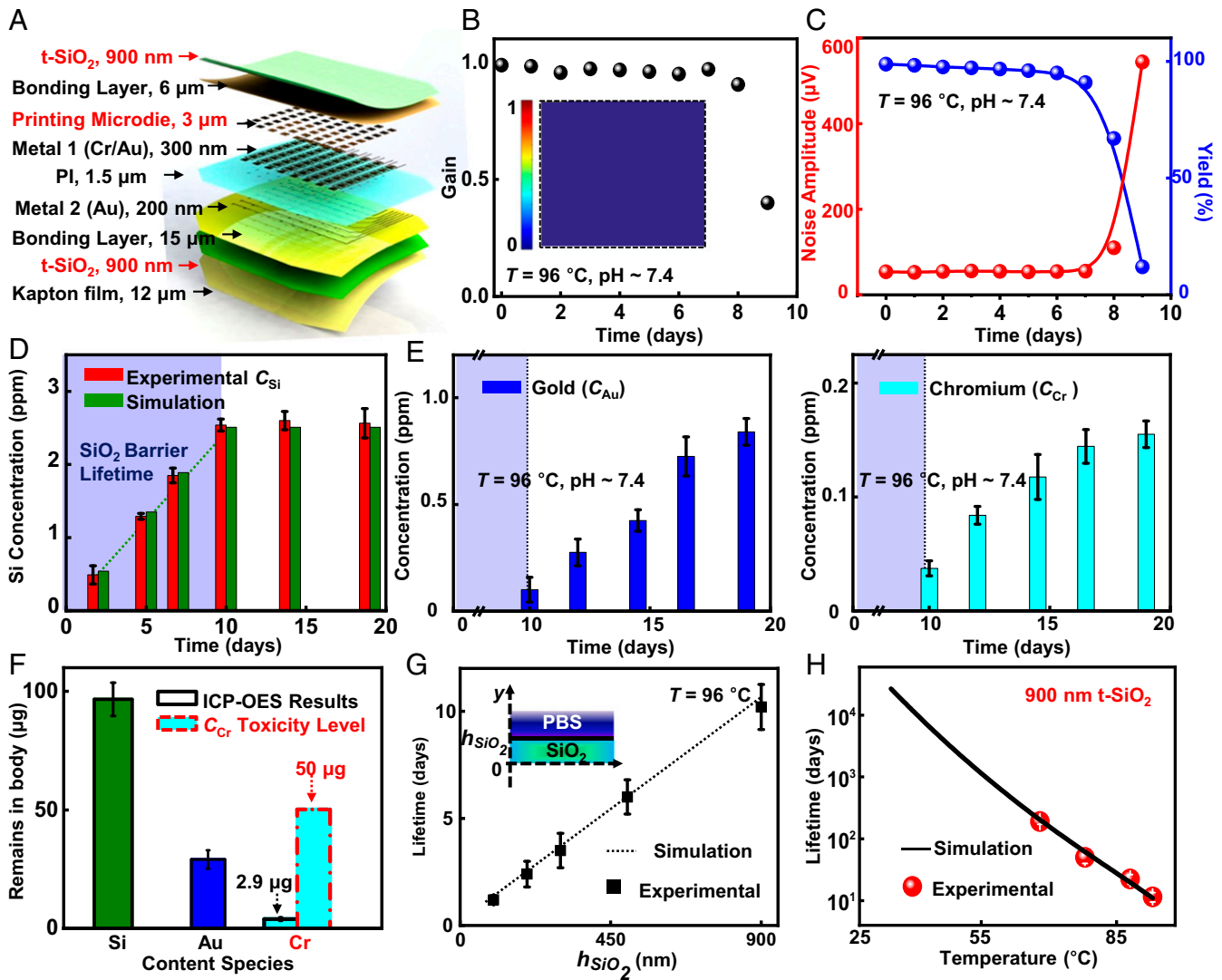
Fig. 5. Chronic stability and biocompatibility assessments. (A) Exploded-view schematic illustration of the layer configuration for an 8 \times 8 array of printed microdie for multiplexed addressing. (B and C) In vitro results of an active system during soak tests at 96^\circ\text{C} , including gain, noise amplitude, and yield. Inset is a map of gain after 10-d soaking in 96^\circ\text{C} PBS. (D and E) ICP-OES results. (D) Si concentration in the PBS used for the accelerated tests. The simulated (green) and measured (red) results show a linear relationship with a rate of \sim 0.27 ppm/d, followed by saturation after dissolution of the t-SiO 2 layer. (E) Metal concentration in PBS. Electrode materials such as Au ( Left ) and Cr ( Right ) start to release in PBS solution (from day 10) after dissolution of the t-SiO 2 . (F) Biocompatibility assessment of the active microdie array. (G) Thickness-dependent and (H) temperature-dependent lifetimes of a t-SiO 2 barrier with simulated (line) and measured (symbols) results. Inset in G is the schematic illustration.
