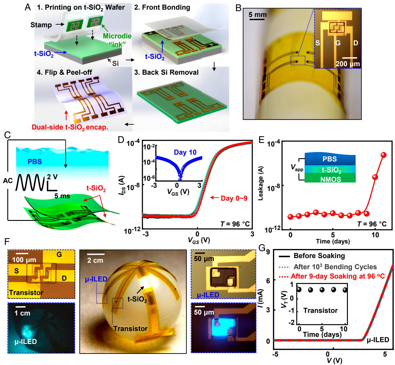
Fig. 3. Integration of electronic/optoelectronic microsystems with thin biofluid barriers of t\text{-SiO}_2 . (A) Schemes for encapsulating systems with t\text{-SiO}_2 . (B) Optical image of a 2 \times 2 transistor array with t\text{-SiO}_2 on both sides. Inset shows a single microdie covered by t\text{-SiO}_2 . (C) Schematic diagram of a system immersed in PBS solution while under electrical bias. (D and E) Accelerated soak test results for a single printed microdie with transfer characteristics (D) and leakage currents (E) collected during immersion in PBS solution at 96^\circ\text{C} and pH 7.4. Insets show the point of catastrophic failure after a stable lifetime and schematic illustrations of the soak test, respectively. The applied voltage ( V_{\text{app}} ) for the leakage analysis is d.c. 3 V. (F and G) Printed cointegration of optoelectronic and electronic components into a system encapsulated by t\text{-SiO}_2 layers. (F) Photograph of printed \mu\text{-ILEDs} and microdie in a starburst-shaped system wrapped over a table-tennis ball. Insets are optical images of a transistor and an \mu\text{-ILED} in off and on states. (G) Bending tests and accelerated soak tests of a system with printed \mu\text{-ILEDs} and transistors. Inset shows transistor performance.
